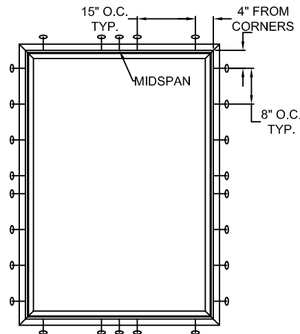
TYPICAL ELEVATION WITH FASTENER SPACING
